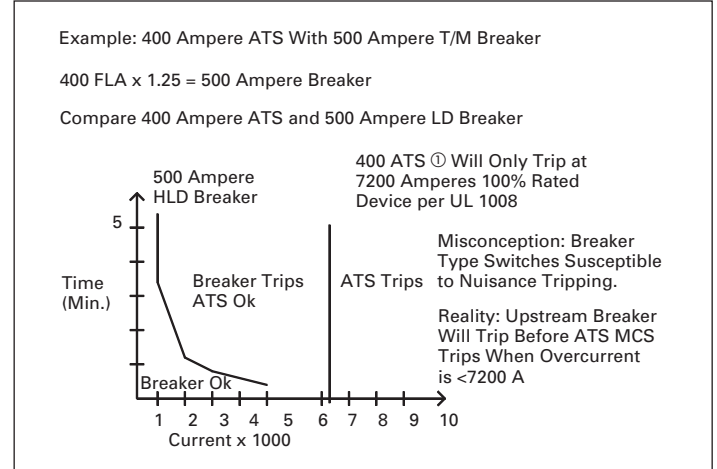
FIGURE 4. BUILT-IN PROTECTION
